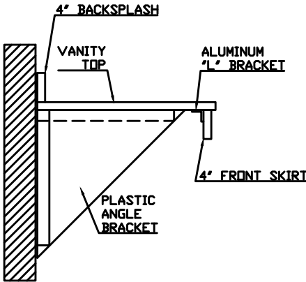
STANDARD STYLE SIDE ELEVATION
