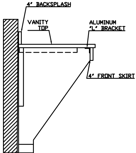
VANITY LEG (OPTIONAL) SIDE ELEVATION
