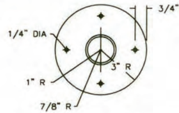
Pedestal Top View
