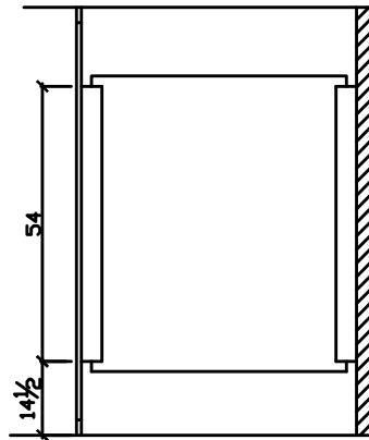
SIDE ELEVATION
