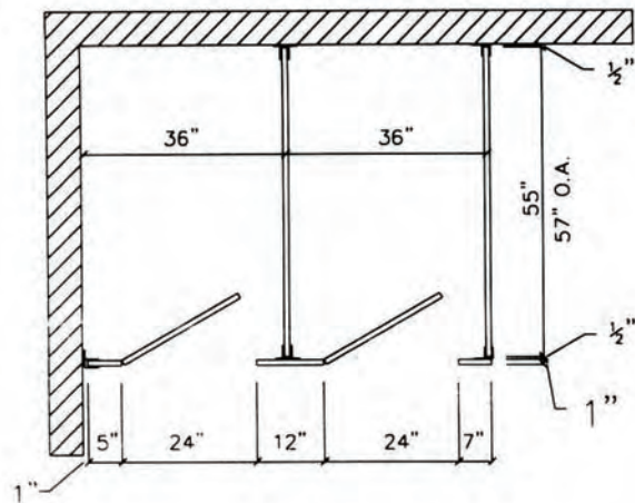
Floor Layout
